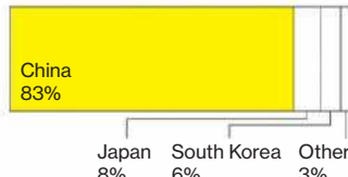
Destinations for Australian iron ore exports in 2016 and 2017
